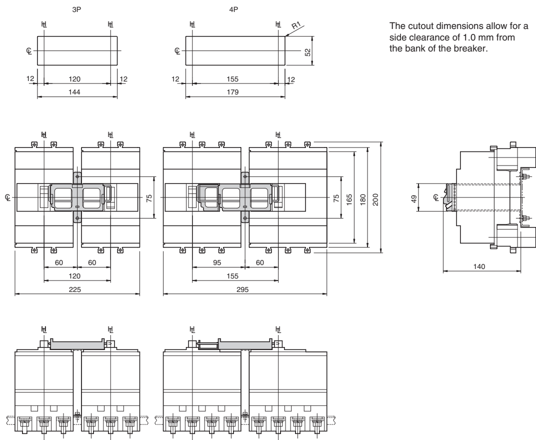
Drilling plan (front view)
