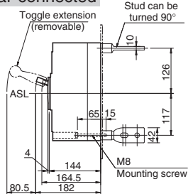
Detail of connecting part
