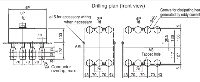
Drilling plan (front view)
