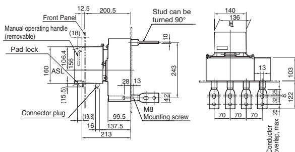
Detail of connecting part
