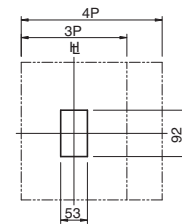
Panel cutout (front view)
