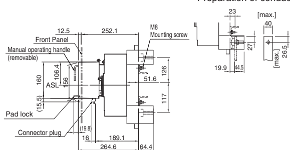
Detail of connecting part and Preparation of conductor
