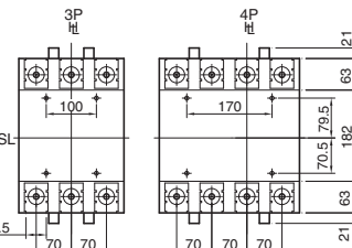
Mounting base (rear view)
