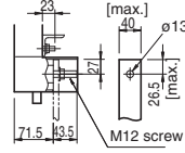
Detail of connecting part and Preparation of conductor
