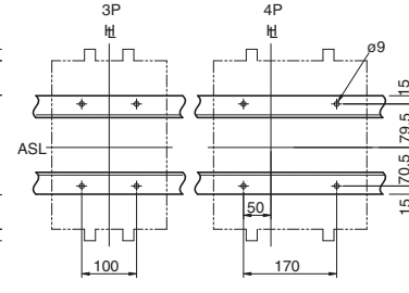
Panel cutout (front view)
