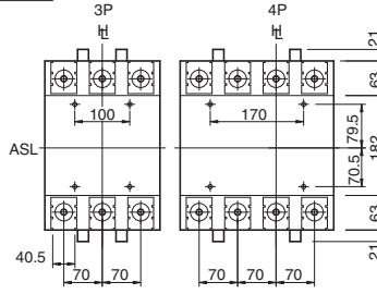
Mounting base (rear view)
