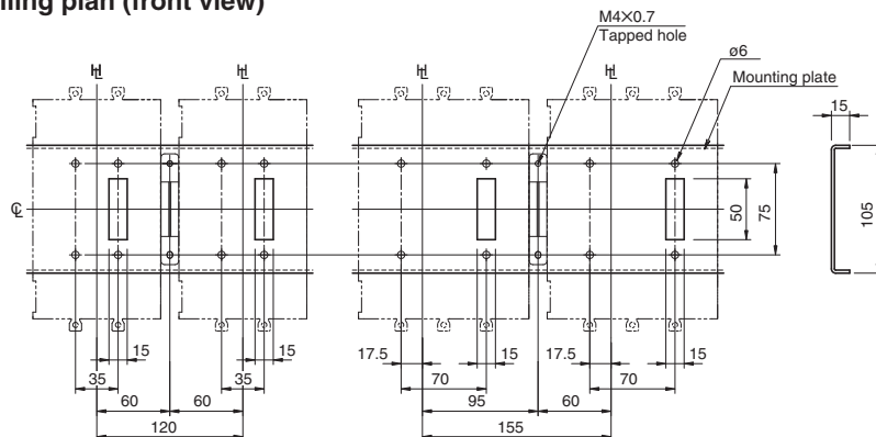
Drilling plan (front view)
