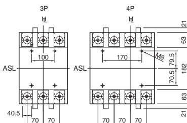
Mounting base (rear view)
